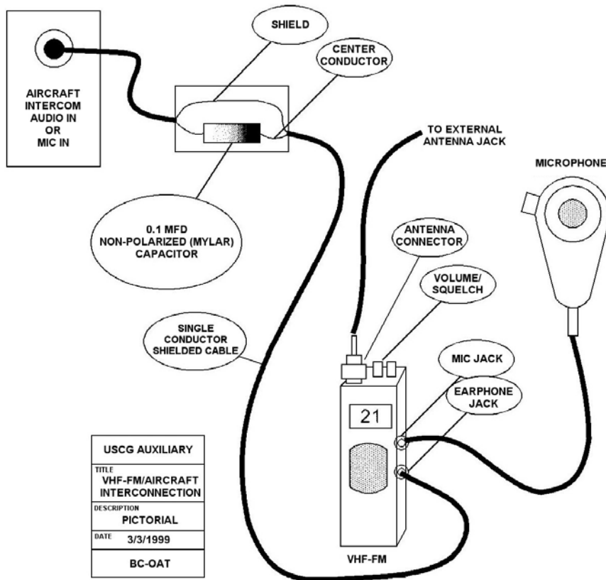
Figure 6-1 Interconnection of VHF-FM Transceiver in Auxiliary Aircraft
