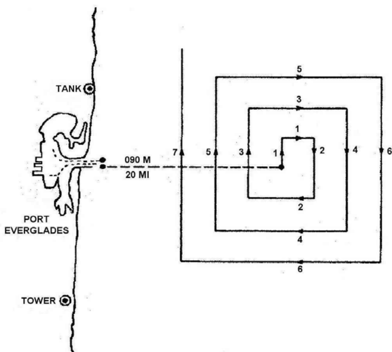
Figure 11-7 Expanding Square Pattern
