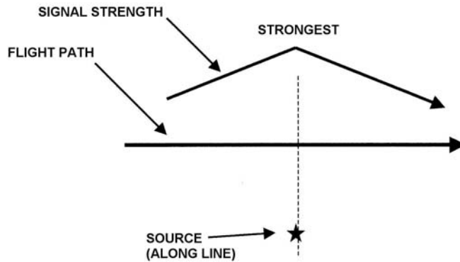
Figure 11-9 Build and Fade Detection
