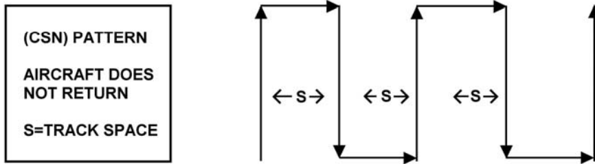
Figure 11-5 Creeping Line Pattern
