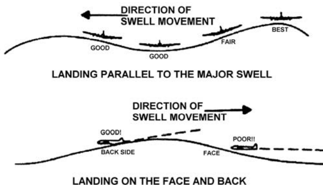
Figure 9-1 Ditching the Aircraft
