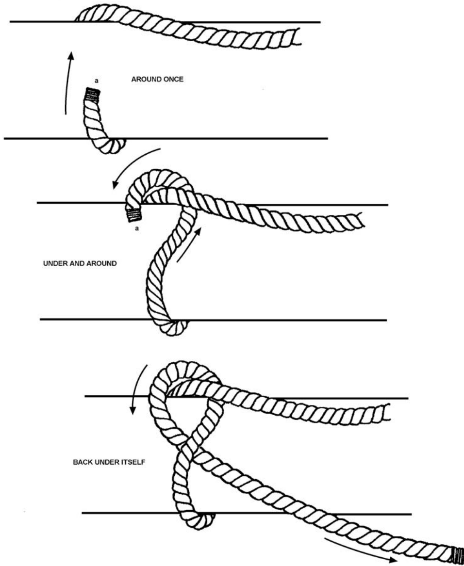
Figure 7-13 Half Hitch
