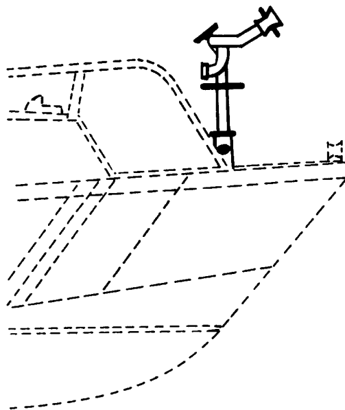
Figure 18-10 Fire Monitor
