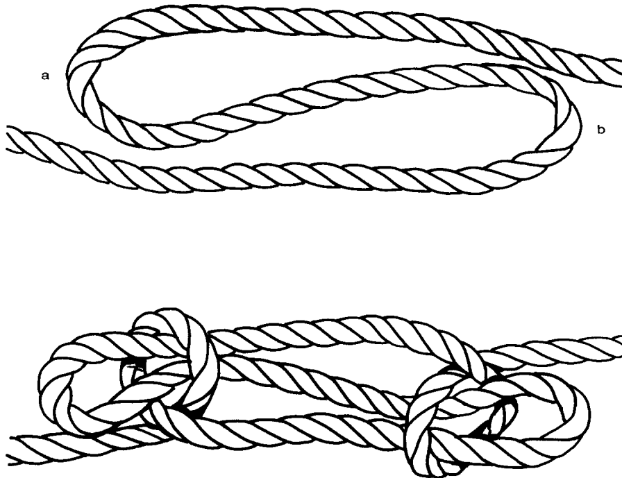
Figure 7-25 Sheepshank
