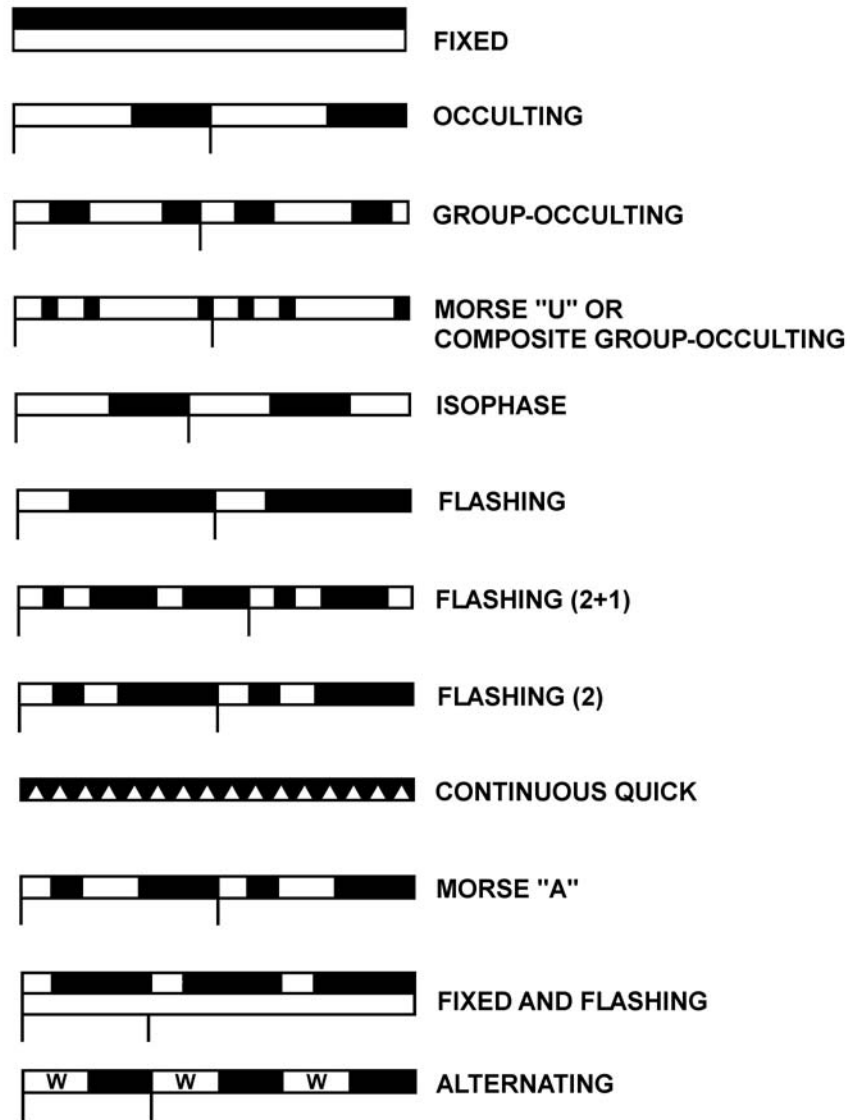
Figure 13-4 Light Characteristics
