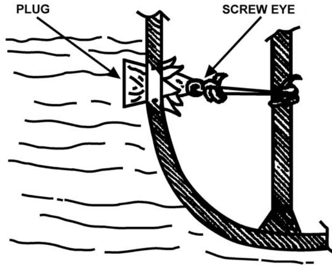
Figure 18-25 Screw Eye
